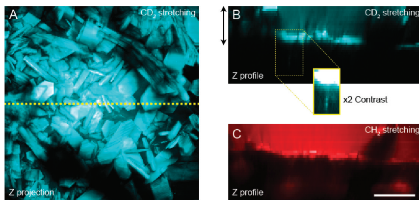
Figure 6. Crystal formation on the skin surface 25 min post-topical application of a solution of ibuprofen in PG. (A) Maximum intensity depth projection (of the upper \sim 30\ \mu\text{m} ) with SRS contrast at 2120\ \text{cm}^{-1} . (B) Depth projection down the yellow dotted line in panel (A) again showing contrast for deuterated ibuprofen. Crystal formation on the tissue surface and some penetration down the hair shaft (inset) are seen. (C) \text{CH}_2 stretching image from the same region showed the bright SC and very clear contrast from the undeuterated PG above the SC. Scale bar = 50\ \mu\text{m} .
